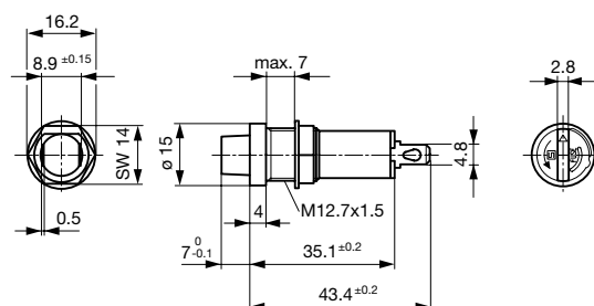
Variant Fingergrip 0031.3911
