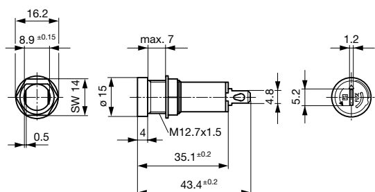
Variant 0031.3901
